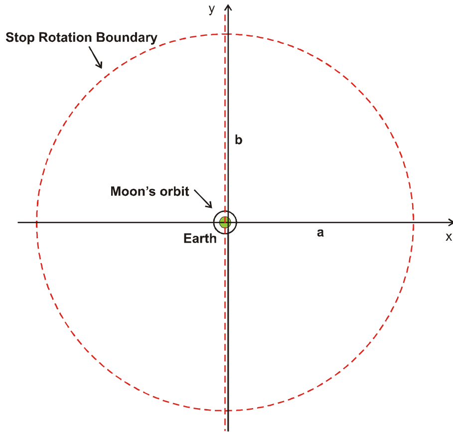
Moon's orbit relative to the Stop Rotation Boundary
